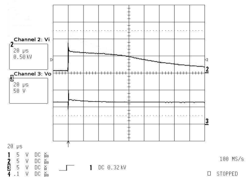
Figure 6 : LGDS-50-Q-K 1800V Spike Response
