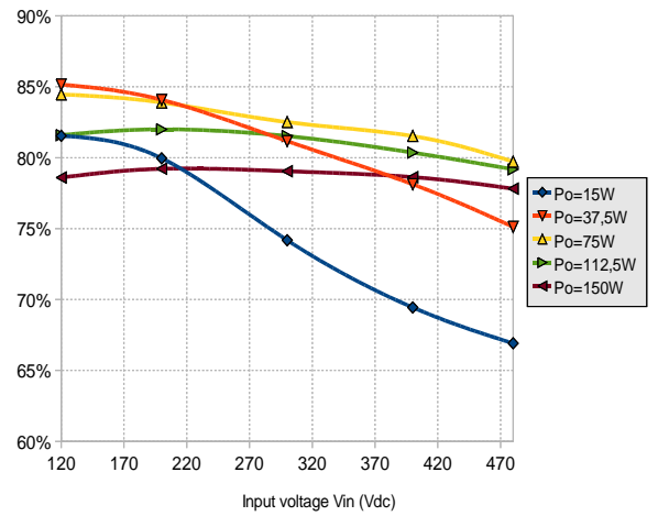
Efficiency versus input Voltage MGDS150TC
