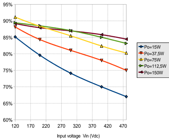
Efficiency versus input Voltage MGDS150TI
