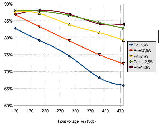
Efficiency versus input Voltage MGDS150TF
