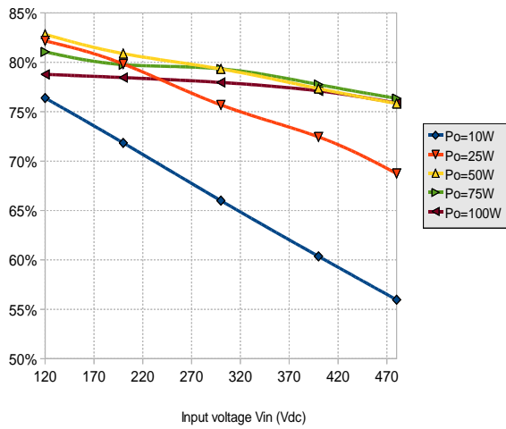
Efficiency versus input Voltage MGDS150TB
