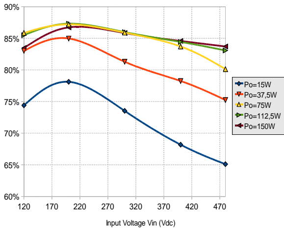
Efficiency versus input Voltage MGDS150TE
