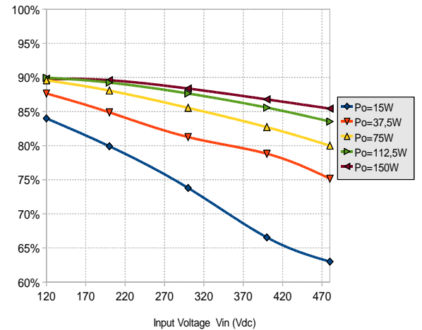
Efficiency versus input Voltage MGDS150TJ
