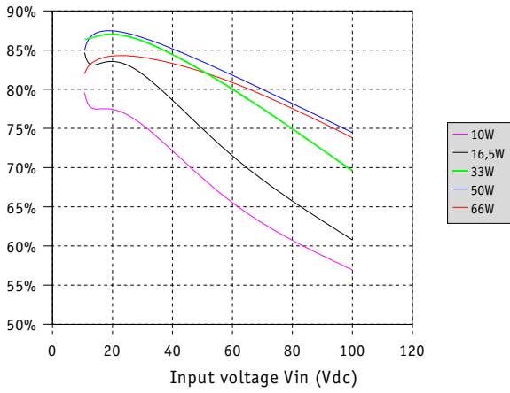
Fig 1 : Typical efficiency MGDS-100-M-B at 25°C
