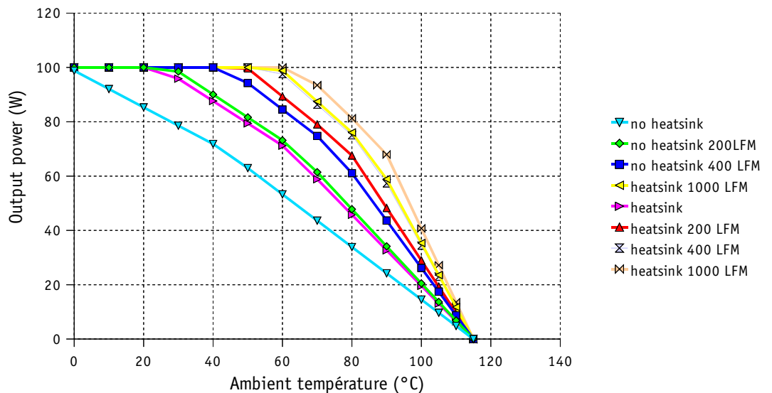
MGDM-100 Series Thermal Curves
