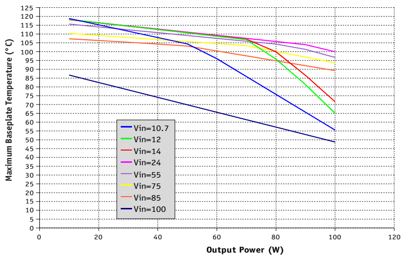
MGDM-100 Series Maximum Baseplate Temperature Versus Output Power
