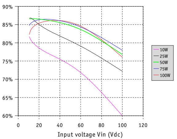
Fig 3 : Typical efficiency MGDS-100-M-E at 25°C
