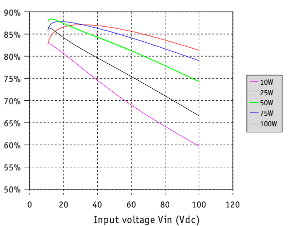
Fig 5 : Typical efficiency MGDS-100-M-26 at 25°C
