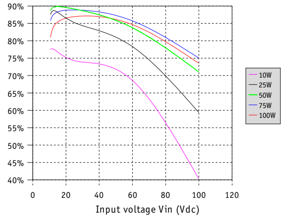
Fig 2 : Typical efficiency MGDS-100-M-C at 25°C
