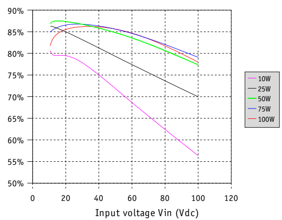
Fig 4 : Typical efficiency MGDS-100-M-F at 25°C
